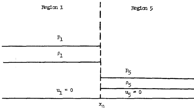
FIG. 2. Shock tube at t = 0 .
